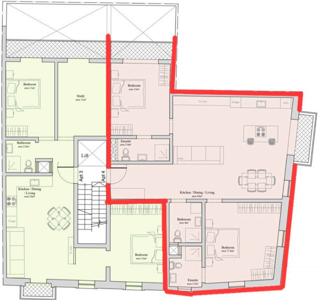
Second floor Floor Plan Scale 1:100
