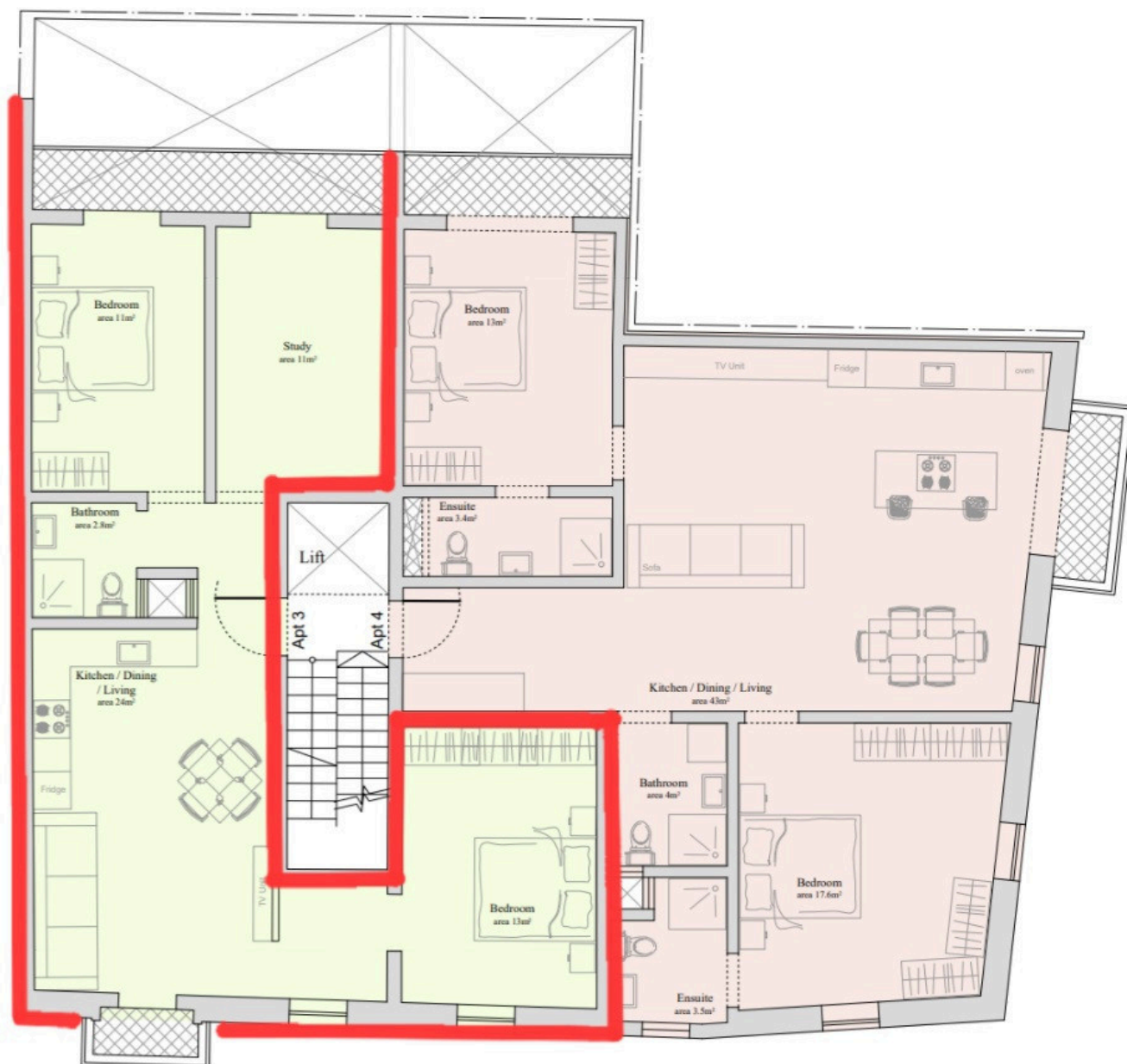
Second floor Floor Plan Scale 1:100
