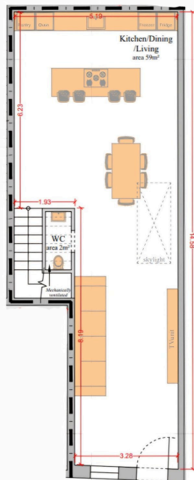
Ground Floor Plan Scale 1:100
