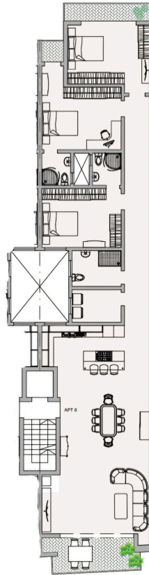
SECOND FLOOR PROPOSED SCALE 1:100
