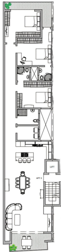
FIRST FLOOR PROPOSED SCALE 1:100
