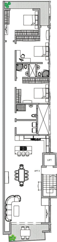
FIRST FLOOR PROPOSED SCALE 1:100
