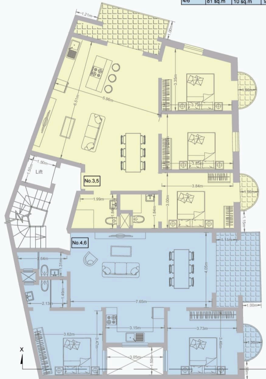
PROPOSED SECOND & THIRD FLOOR PLAN SCALE 1:100
