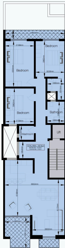
LEVEL 2 SCALE 1:100
